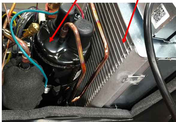
4035852 Compressor
